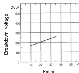
(3) Breakdown voltage
