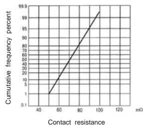
(2) Contact resistance
