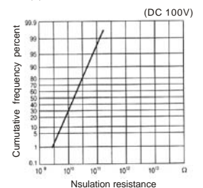
(4) Insulation resistance
